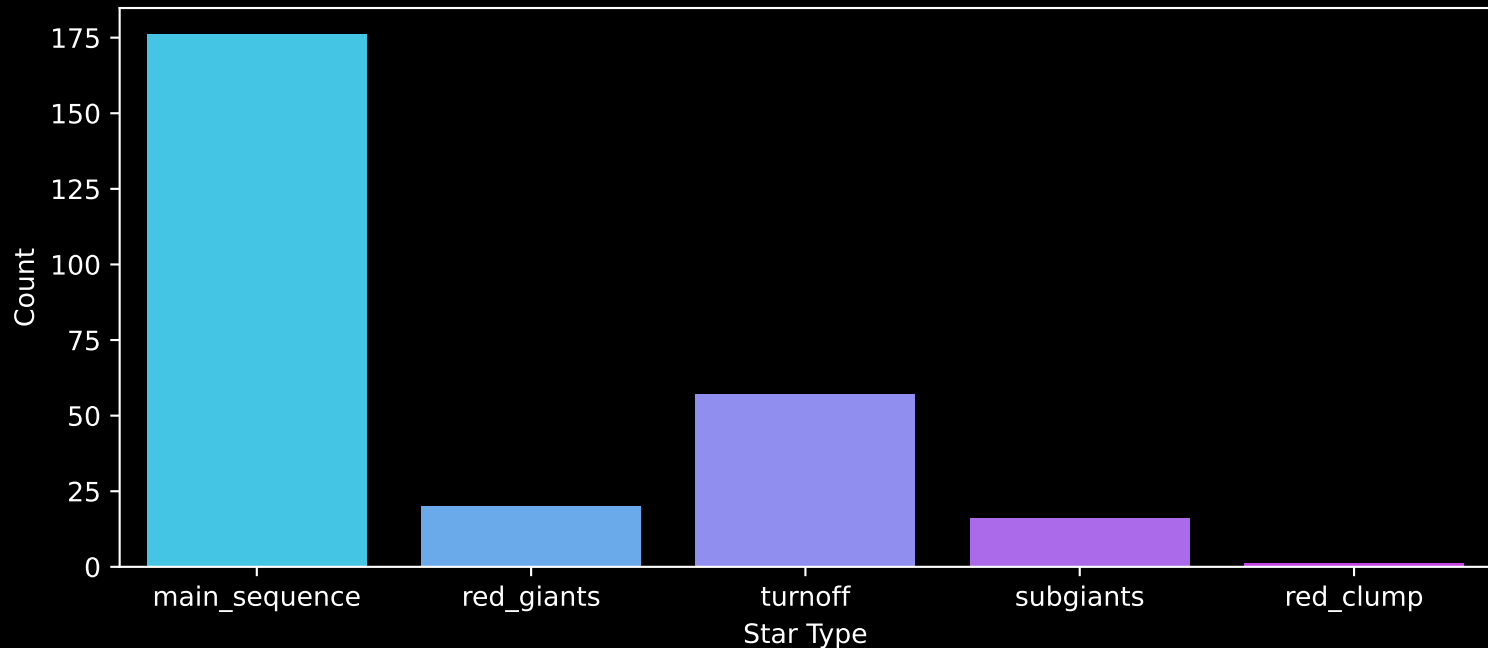
GALAH DR4 Field: [6834] Count plot of Star Type
