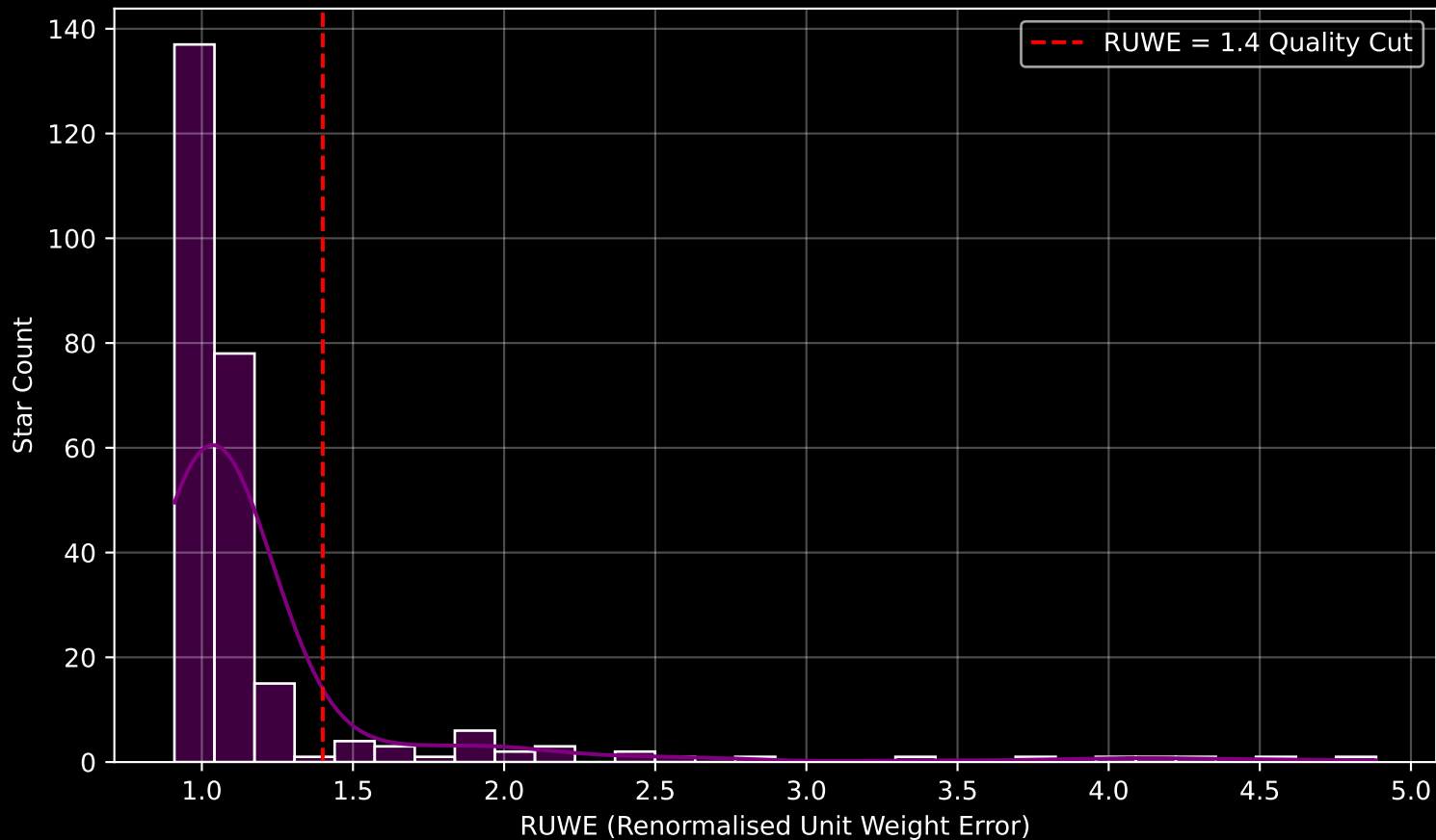
GALAH DR4 Field [6834] RUWE Distribution (n= 261)
